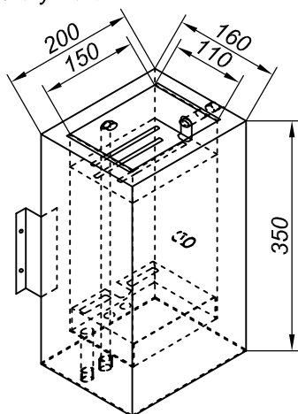
No.83 Sterylizator
