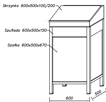
Pulpit 600x500x1200
