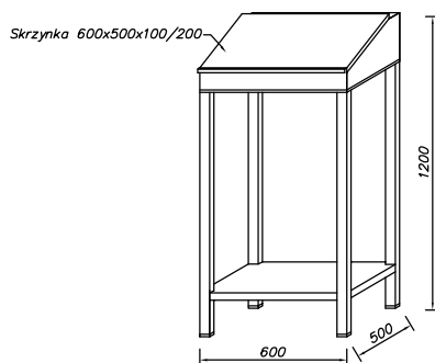
Pulpit 600x500x1200
